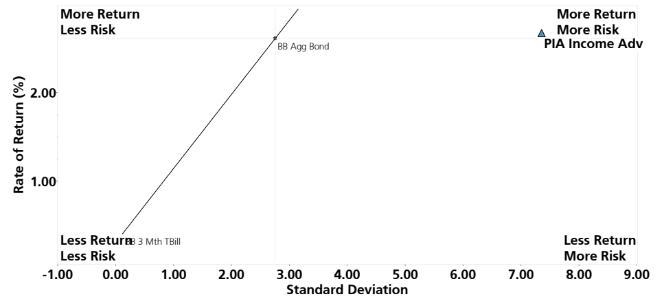
Since Inception
