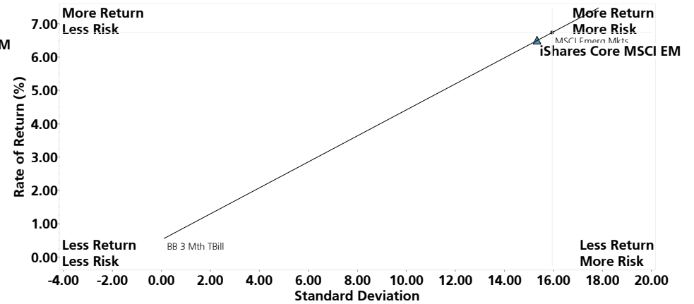
Since Inception
